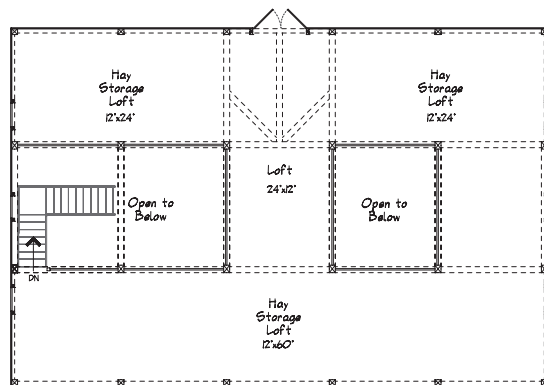
LOFT LEVEL
